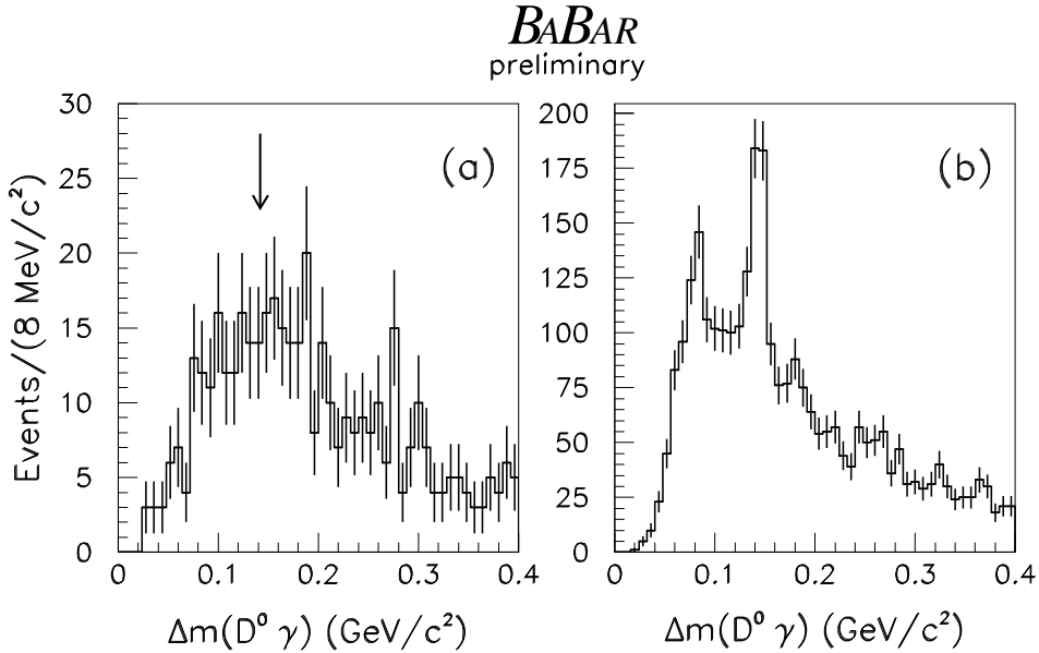
Figure 3: Spectra of \Delta m(D^0\gamma) \equiv m(D^0\gamma) - m(D^0) for (a) all events inside and (b) D^0 \rightarrow K^-\pi^+, \bar{D}^0 \rightarrow K^+\pi^- events outside the exclusive ISR region. The arrow indicates the expected position of D^{*0} .
